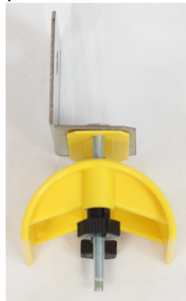
FTSW-EDFL: End Clamp to use with flat cable
